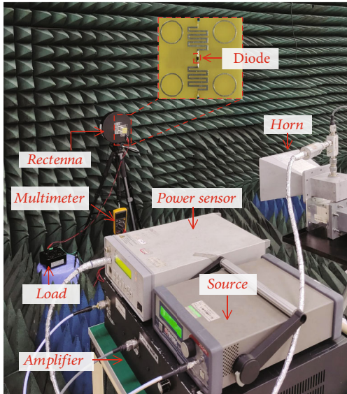
FIGURE 5: Fabricated rectenna and measurement in an anechoic chamber.
